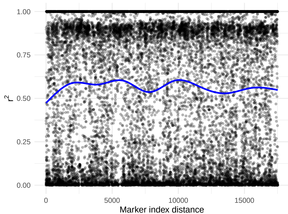
LD Decay Plot
